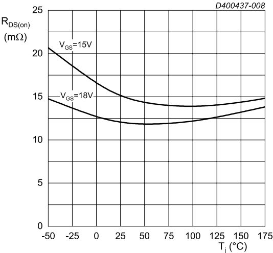
I_{DS} = 75\text{ A}; t_p < 200\text{ }\mu\text{s} Fig. 8. Drain-source on-state resistance as a function of junction temperature
